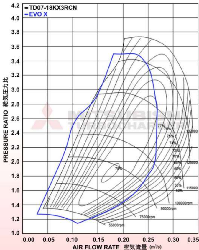
COMPRESSOR MAP
